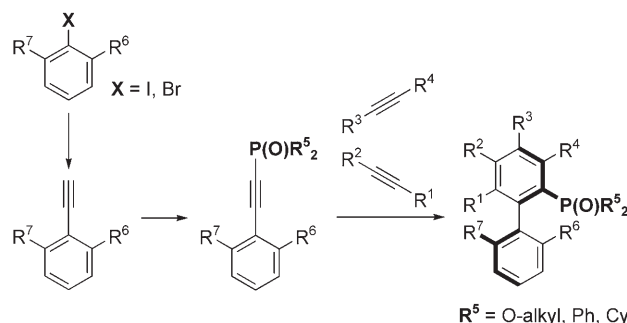
Scheme 2. Synthesis of tetra-ortho-substituted axially chiral biaryl phosphonates and phosphine oxides through the asymmetric assembly of aromatic rings. Cy = cyclohexyl.
