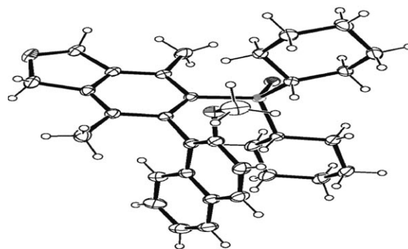
Figure 1. ORTEP diagram of ( S )-(+)- 3ae (product of Table 1, entry 10; R 1 = Me, R 2 = Cy, Z = O). C white, P gray, O black.
