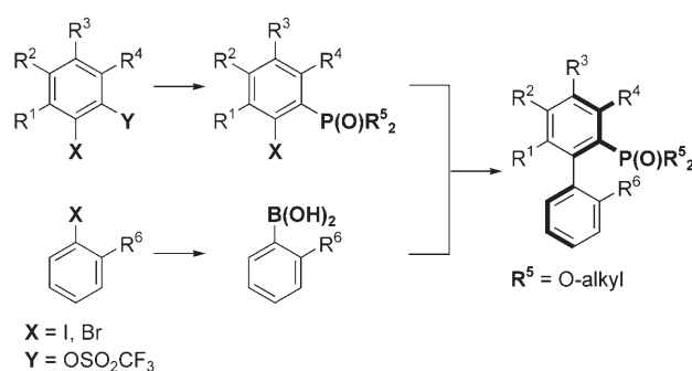
Scheme 1. Synthesis of tri-ortho-substituted axially chiral biaryl phosphonates through asymmetric aryl-aryl cross-coupling.
